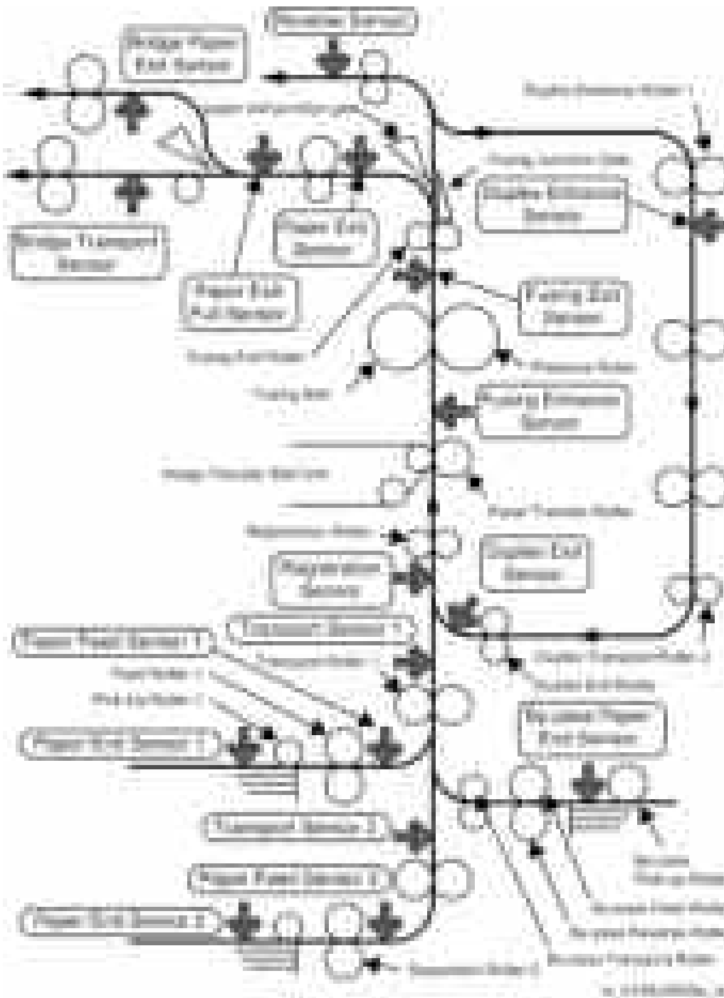
Transport Roller Drive Source
